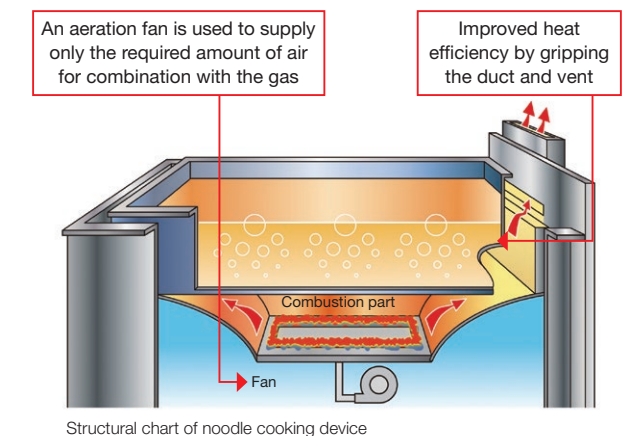
Structural chart of noodle cooking device
